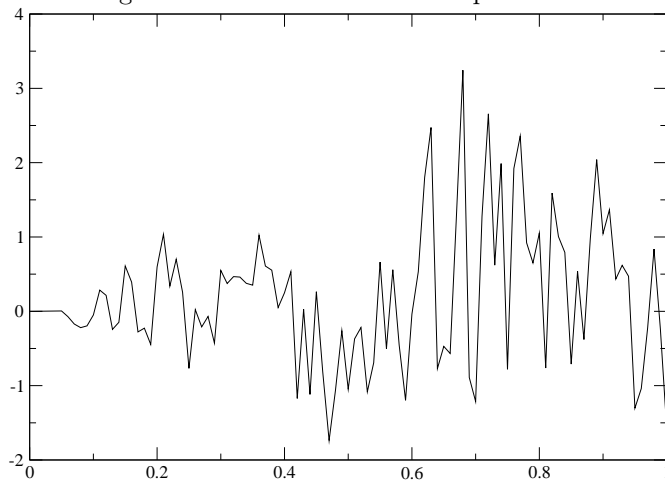
Figure 5.10: Field vs. source amplitude with nonlinear material
