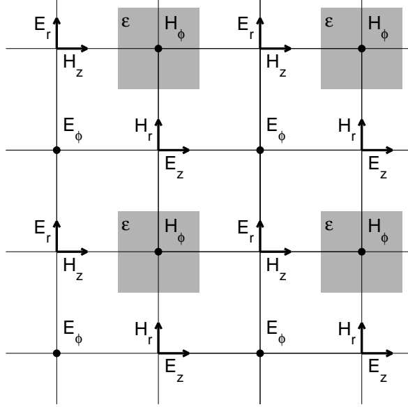
Figure 1.1: Yee lattice in cylindrical coordinates.
