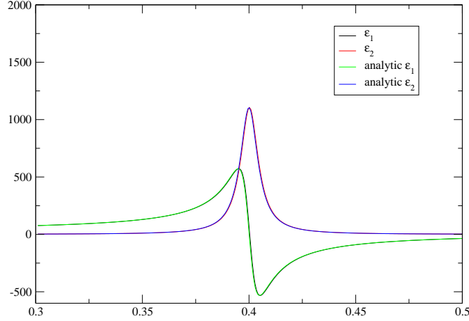
Figure 5.7: Epsilon of a polaritonic material.
