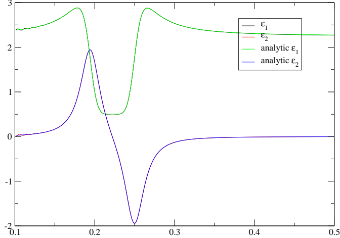
Figure 5.8: Dielectric function of a material with loss and gain.
