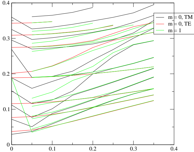
Figure 5.3: Omniguide band structure.
