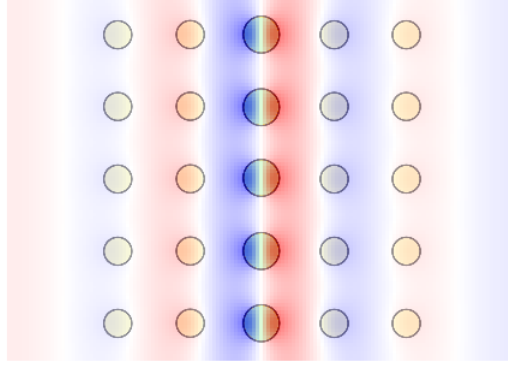
Figure 3-8: Snapshot of the “ \pi -like” defect mode centered about \omega = 0.346(2\pi c/a) .
