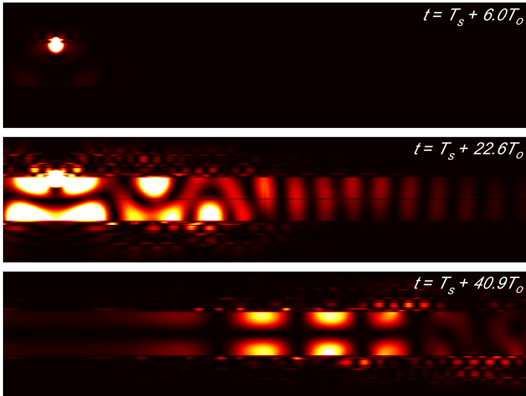
Figure 2-9: Snapshots of the distribution of electrical power in the waveguide for a single dipole source on the inner surface pointing in the \rho direction.
