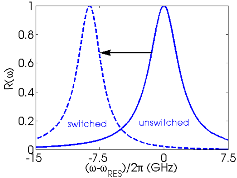
Figure 6-4: Waveguide reflection with (dashed) and without (solid) a control photon, demonstrating lossless switching, where a higher quality factor has made the resonant peaks narrow enough to be shifted by more than their full width at half maximum by a single photon ( \Gamma_w = 3 GHz, g_{13} = 20.5 GHz, \Omega_c = 30 GHz, \Gamma_3 = 0 , g_{24} = 30 GHz and \Delta\tilde{\omega}_{24} = 20 GHz).
