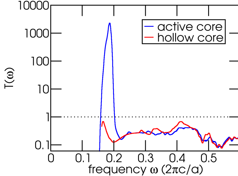
Figure 3-12: Transmission for a cylindrical photonic crystal structure with and without active material at the core. Notice the slight decrease in transmission at \omega \approx 0.4(2\pi c/a) and the sharp increase in transmission about \omega \approx 0.186(2\pi c/a) for the active material.
