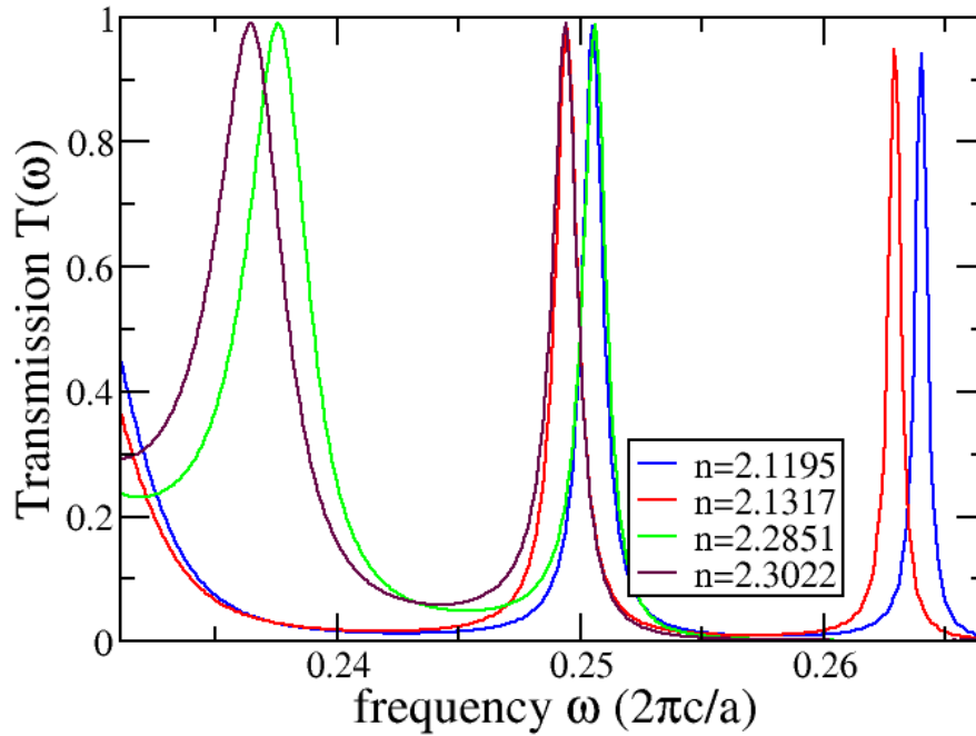
Figure 5-5: Transmission versus frequency for a single device with four different electrooptic material refractive indices. These indices (shown in the legend) are chosen such that all the half-maxima coincide, thus yielding a phase shift of \pi/2 between each device.
