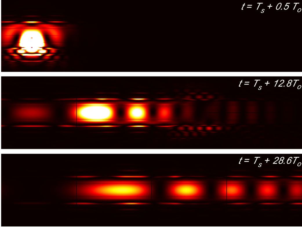
Figure 2-18: Snapshots of the distribution of electrical power in the waveguide for a single dipole source, oriented along z , on the inner surface of a cell with a coating of low-index material ( n = 1.3 ) extending from \rho = 1.2a to \rho = 2.144a .
