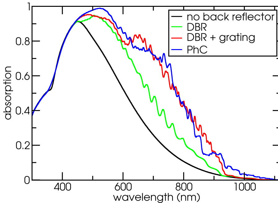
Figure 4-10: Absorption vs. wavelength at normal incidence for four 2\ \mu\text{m} -thick Si cell designs: no back reflector, plain DBR, a DBR plus a 1D-periodic grating, and finally, a 2D photonic crystal of air holes in silicon. The last two designs consist of six complete layers. The photonic crystal-based design yields the highest efficiency.
