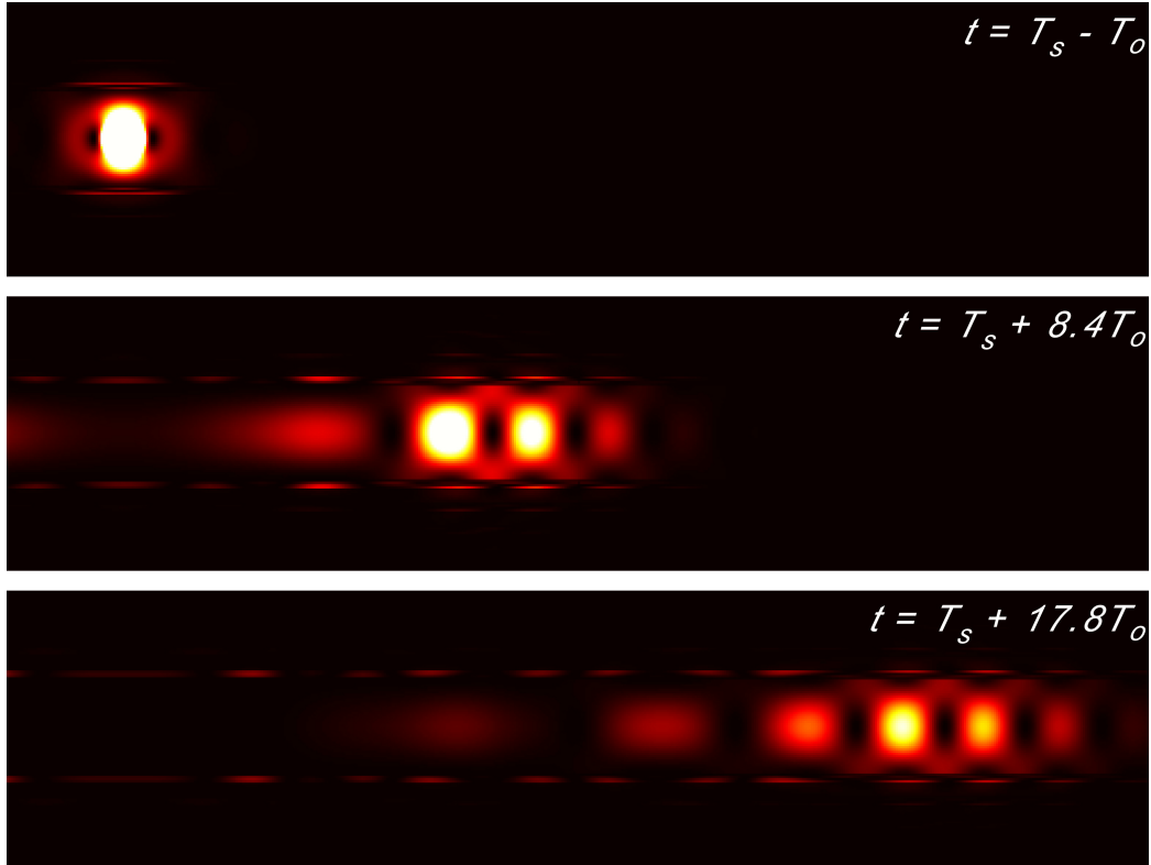
Figure 2-4: Snapshots of the distribution of electrical power in the waveguide for a single dipole at the center of the hollow core. Times are given here and in other figures relative to the time of peak emission, T_s , in units of the period of the central frequency, T_o .
