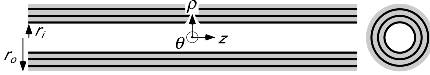
Figure 2-3: Waveguide used in simulations, consisting of 3 bilayers of tellurium ( n = 4.6 ) and polystyrene ( n = 1.6 ). The core is hollow and made of air (the inner radius – the distance from the center to the innermost cladding layer – is given by r_i = 2.144a ; the outer radius – the distance from the center to the outermost cladding layer – is given by r_o = 5.144a ).
