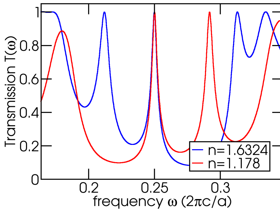
Figure 5-3: Transmission as a function of frequency for two values of the index of the microcavity, n_c = 1.178 and n_c = 1.6324 , chosen to shift two different resonances to the same central frequency \omega = 0.25(2\pi c/a) .
