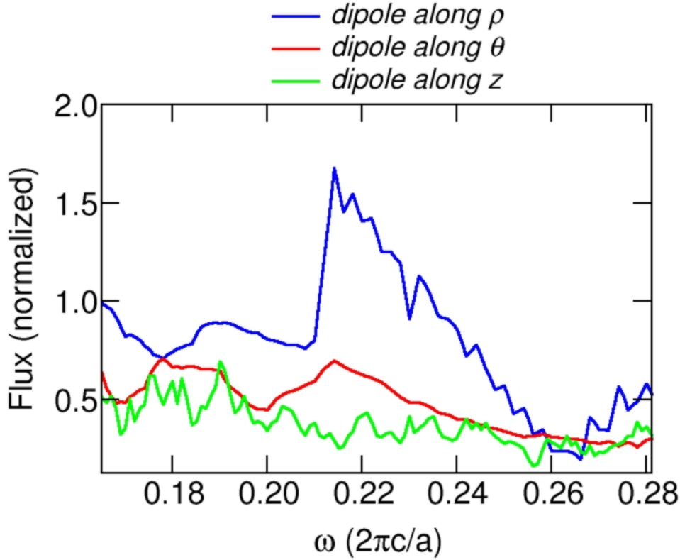
Figure 2-8: Flux spectrum for dipoles on the inner surface of the hollow core, oriented in the \rho , \theta , and z directions, normalized by the flux of a dipole in vacuum.
