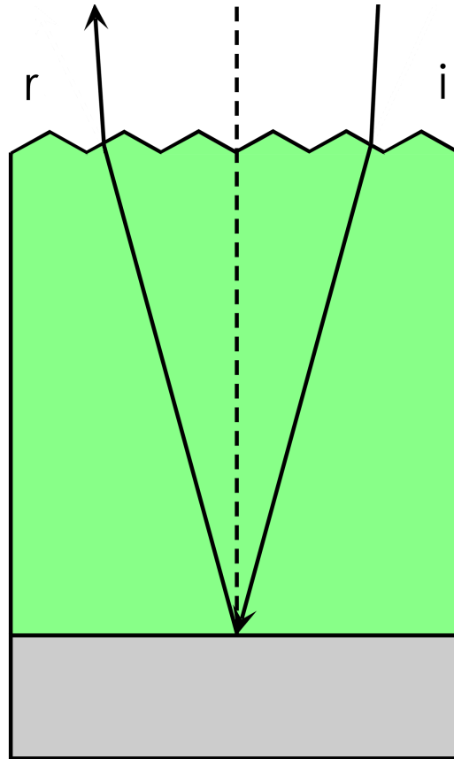
Figure 4-1: Illustration of conventional solar cell light trapping. Note that the front-surface texturing increases the effective path length via refraction into an oblique angle.
