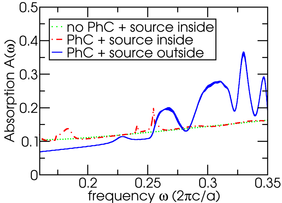
Figure 4-9: Absorption versus frequency for TE modes at oblique incidence for a photonic crystal consisting of 3 layers of a 2D lattice of air holes with r = 0.55a and period 1.375a .
