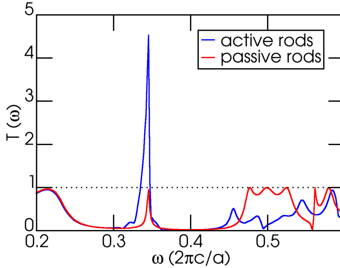
Figure 3-7: Transmission for active and passive versions of the geometry shown in Fig. 3-6. Notice the sharp enhancement of the defect mode peak in the gap to above 100%, the signature of a gain medium.
