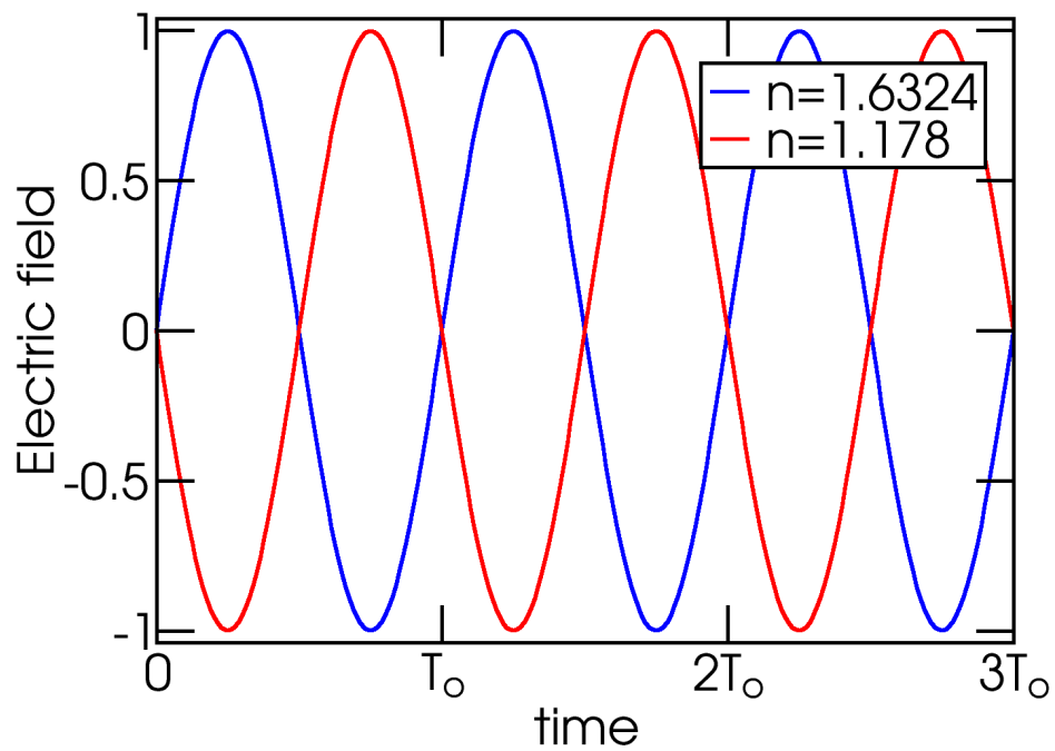
Figure 5-4: Electric fields as a function of time at a point opposite the source for two values of the index of the microcavity, n_c = 1.178 and n_c = 1.6324 . The two outputs are \pi out of phase with respect to one another.
