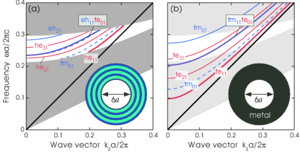
Figure 1-3: Projected bandstructure for (a) an omniguide with a diameter of 6 periods of the omnidirectional reflector, and (b) for a metallic waveguide with the same diameter. Just like in the metallic waveguide, modes in the omniguide observe a quadratic dispersion, for omnidirectionally reflected frequencies (adapted from Ref. [3]).
