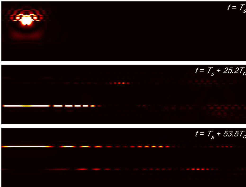
Figure 2-11: Snapshots of the distribution of electrical power in the waveguide for a single dipole source on the inner surface pointing in the z direction.
