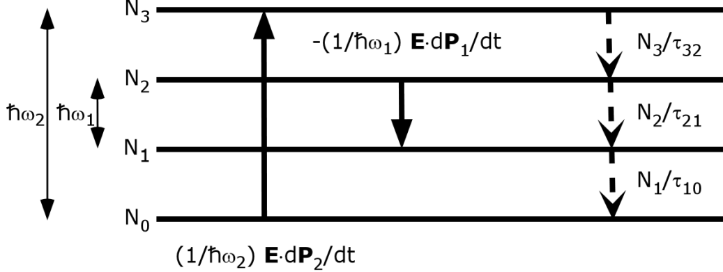
Figure 3-1: Relationships between energy levels in the four-level atomic system used in this chapter. Straight lines correspond to radiative transitions; dashed lines correspond to non-radiative transitions.
