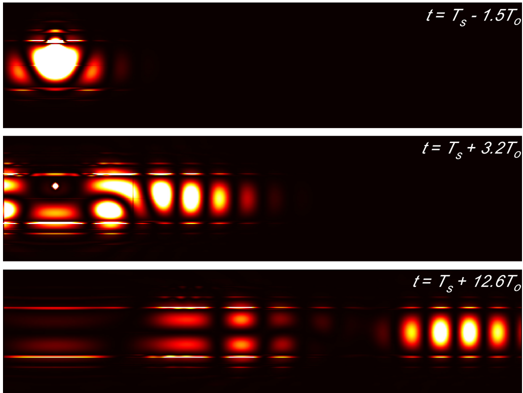
Figure 2-15: Snapshots of the distribution of electrical power in the waveguide for a single dipole source near the inner surface ( \rho = 1.2a , r_i = 2.144a ) pointing in the \theta direction.
