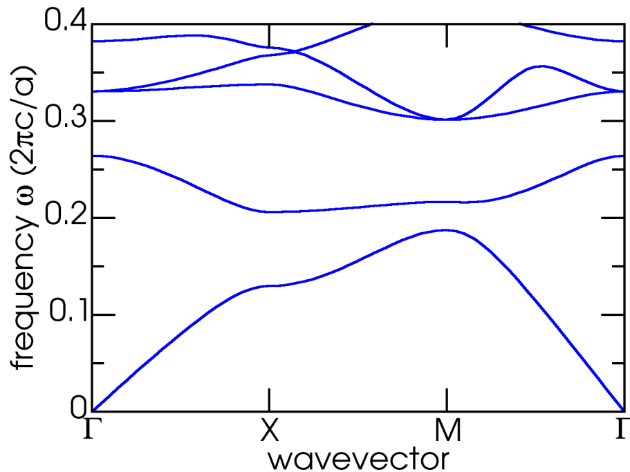
Figure 4-7: Bandstructure for tranverse electric (TE) modes in a photonic crystal consisting of an infinite 2D square lattice of air holes in c-Si with period 1.375a and radius r = 0.55a .
