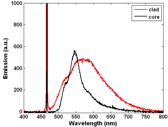
Figure 2-1: Experimental measurement of the flux spectrum for spontaneously emitted light collected in the core and cladding regions of an omniguide fiber (adapted from Ref. [5]).
