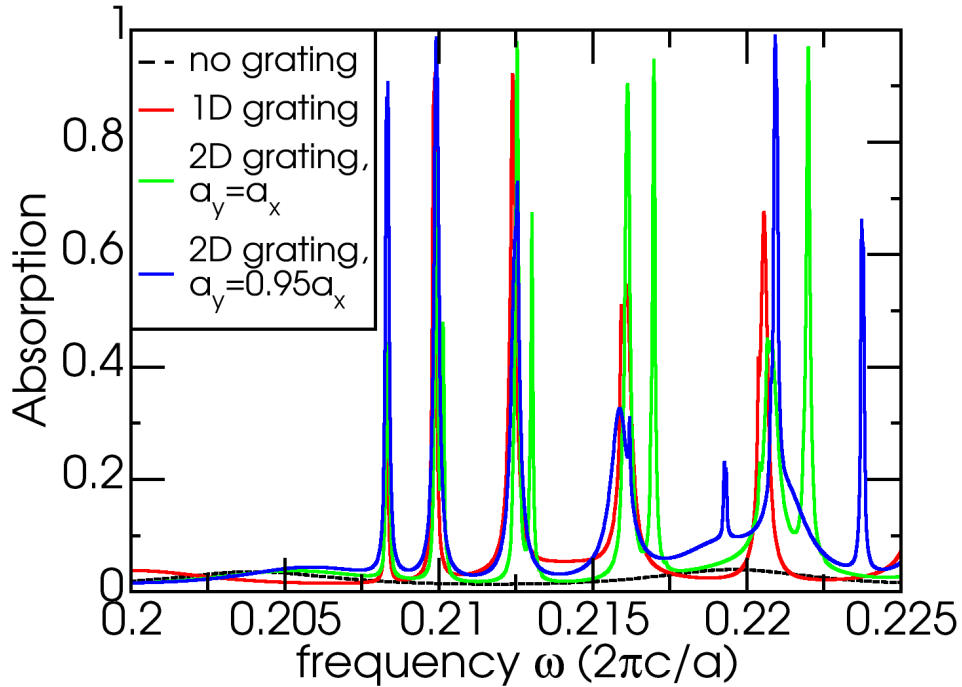
Figure 4-3: Absorption versus frequency of a 2 \mu\text{m} -thick layer of c-Si, with several different metal reflectors on bottom: one which is planar, one with 1D etching, and two with 2D “checkerboard” etching patterns and slightly different ratios of the x- and y-periods. All gratings have a square etch with a fill factor of one-half in each direction.
