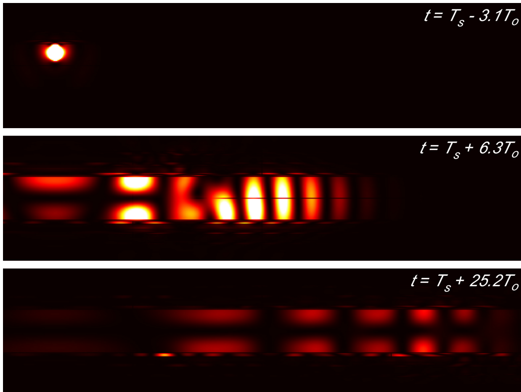
Figure 2-14: Snapshots of the distribution of electrical power in the waveguide for a single dipole source near the inner surface ( \rho = 1.2a , r_i = 2.144a ) pointing in the \rho direction.
