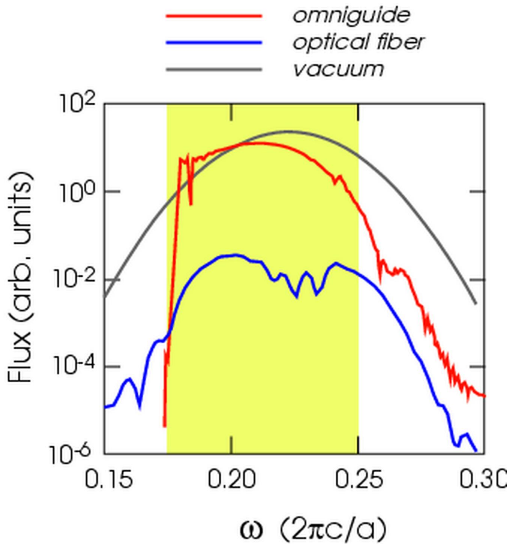
Figure 2-5: Flux spectrum for a dipole at the center of the hollow core, plus data for a hollow glass fiber ( n = 2.6 ), and the total flux of the dipole in vacuum.
