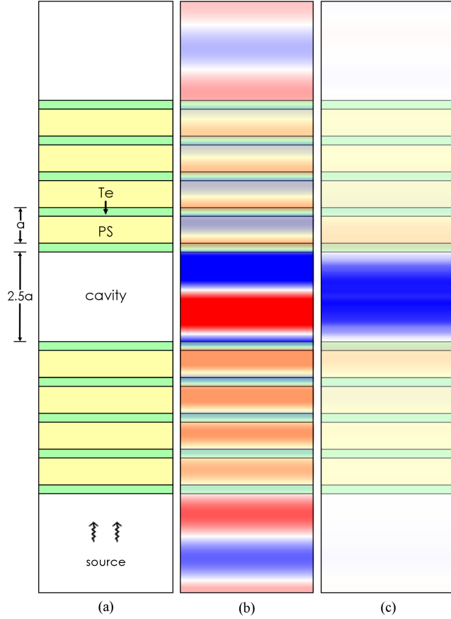
Figure 3-4: Conversion of light from the optical pumping frequency ( \omega = 0.4(2\pi c/a) ) to the stimulated emission frequency ( \omega = 0.2(2\pi c/a) ) in a Fabry-Perot cavity, illustrated in (a). The pump pulse is shown in (b) and the stimulated emission is shown in (c). Green represents high dielectric tellurium, yellow representing lower dielectric polystyrene; blue and red signify positive and negative electric fields, respectively.
