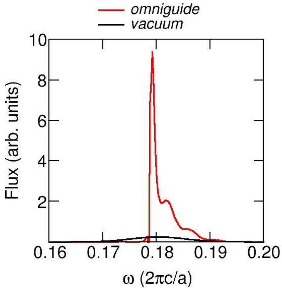
Figure 2-7: Flux spectrum for a dipole at the center of the hollow core, as in figure 2-5, but zoomed in on the region near cutoff.
