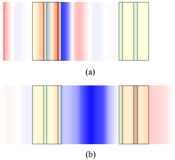
Figure 3-11: Conversion of light at an optical pump frequency into a stimulated emission frequency, as in Fig. 3-10, but in a cross-section through the center of the core along the z -axis.
