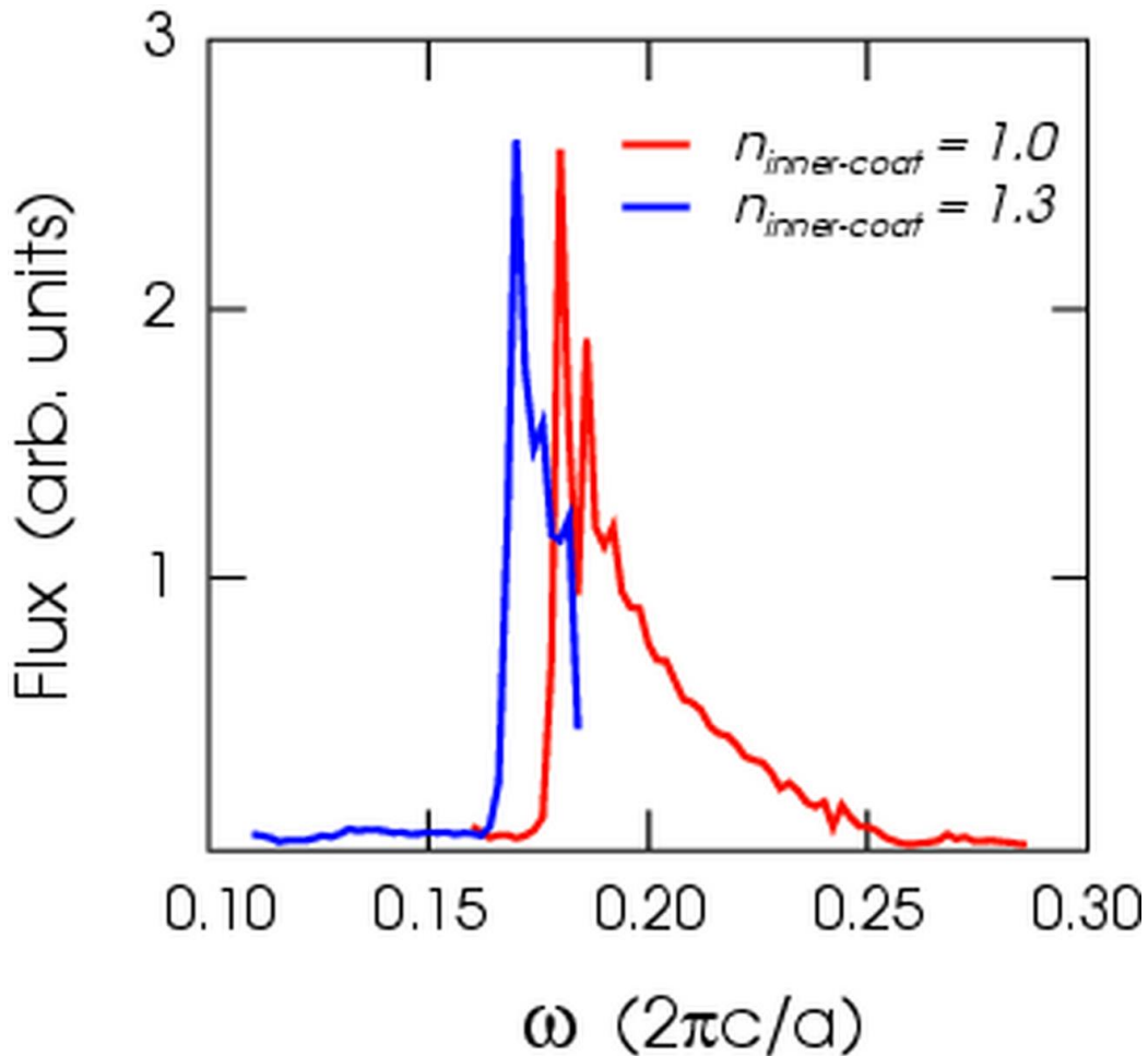
Figure 2-17: Flux spectrum for dipoles oriented along z situated on the inner wall of a medium-sized cell with an inner coating of low-index material ( n = 1.3 ) extending from \rho = 1.2a to \rho = 2.144a .
