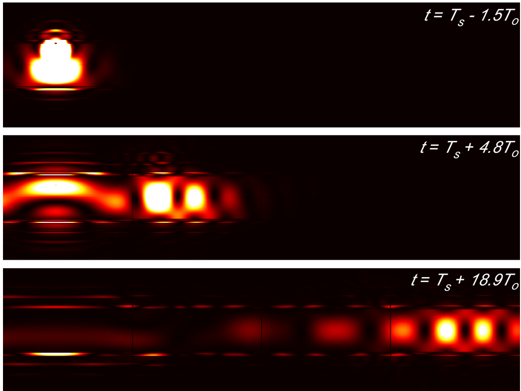
Figure 2-16: Snapshots of the distribution of electrical power in the waveguide for a single dipole source near the inner surface ( \rho = 1.2a , r_i = 2.144a ) pointing in the z direction.
